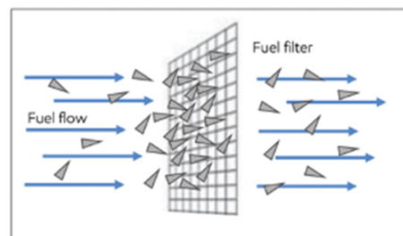
Cold-flow improver modifies the wax crystals into needle-shaped crystals, allowing some wax and fuel to pass through the filter.
